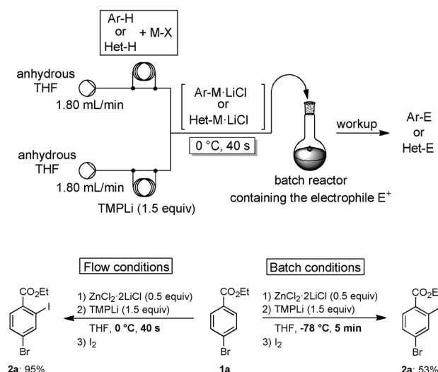
Scheme 2. Continuous-flow setup for in situ trapping metalations using TMPLi in the presence of metal salts ( \text{ZnCl}_2 \cdot 2\text{LiCl} , \text{MgCl}_2 , \text{CuCN} \cdot 2\text{LiCl} , \text{LaCl}_3 \cdot 2\text{LiCl} ) (top) and iodination of ethyl 4-bromobenzoate ( 1a ) using flow and batch conditions for the in situ trapping metalation (bottom).
