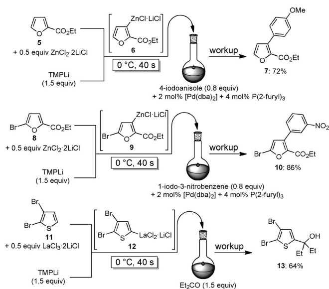
Scheme 3. In situ trapping zincation or lanthanation of functionalized furans or thiophenes using \text{TMPLi} and \text{ZnCl}_2 \cdot 2\text{LiCl} or \text{LaCl}_3 \cdot 2\text{LiCl} in flow mode.
